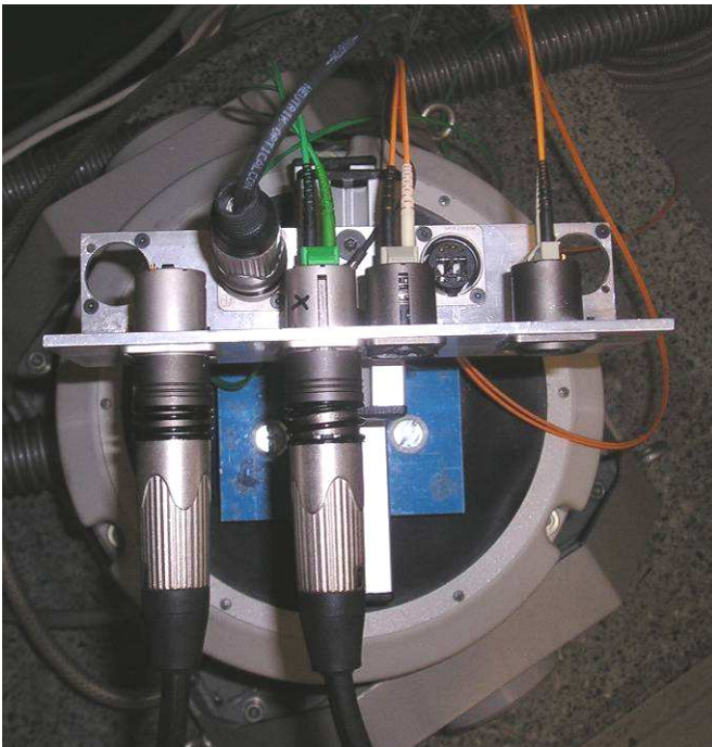
Fig. 3b: Vibration equipment and test cable arrangement
