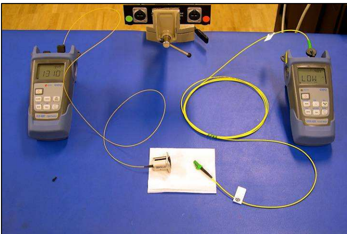
Fig. 22: Test Set-Up
