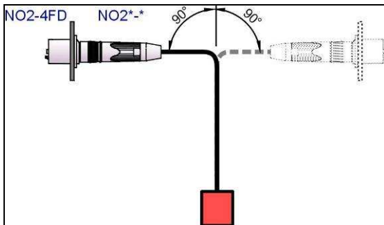
Fig. 18: Principle of Test according to IEC 61300-2-44 (IEC 61300-3-4)
