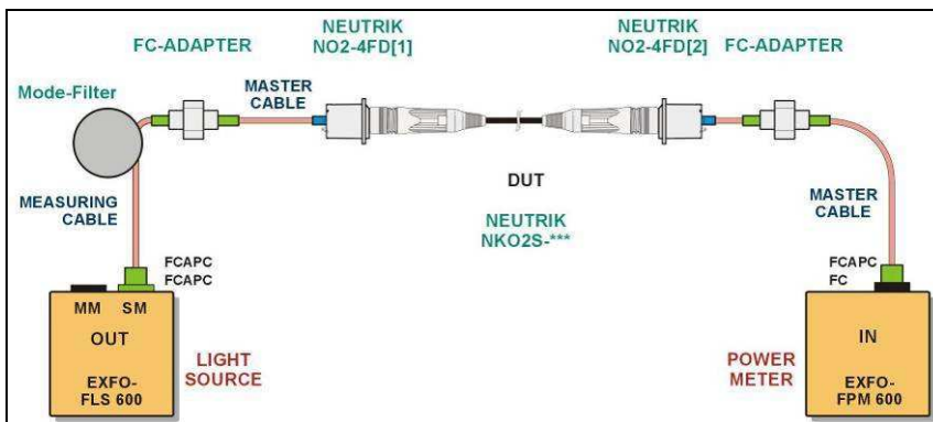
Fig. 2: Simplified measuring arrangement
