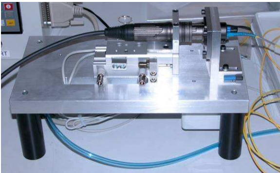
Fig. 7 fixture for 500 and 5000 mating cycles.
