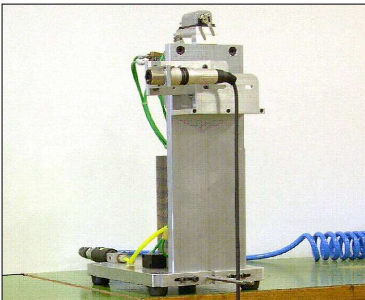
Fig. 19: Test Equipment and Fixture for flexing test
