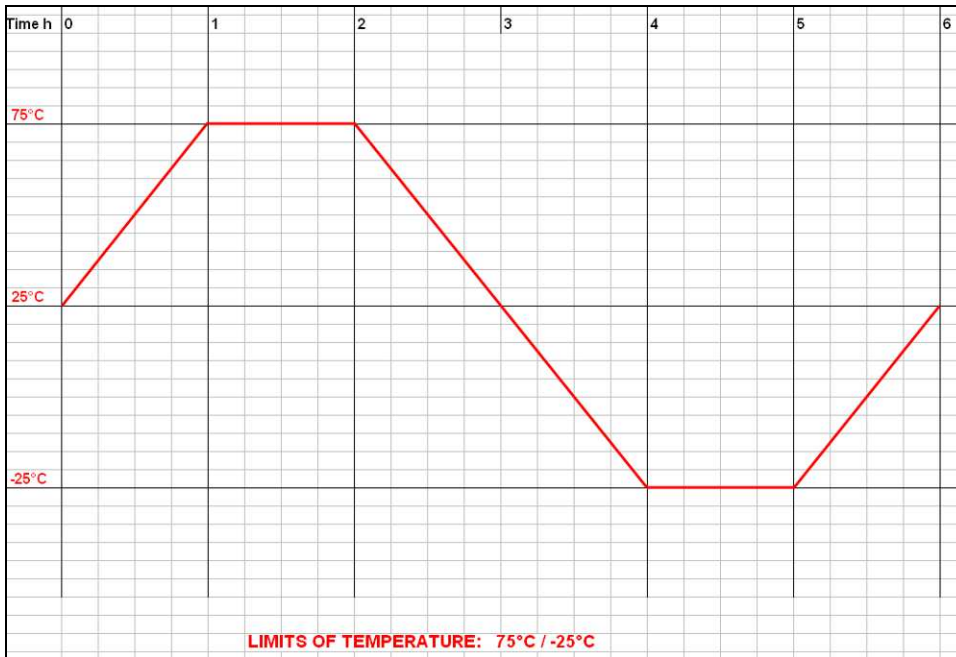
Fig. 17: Profile of temperature
